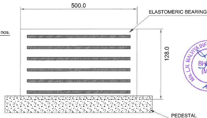
ARRANGEMENT OF BEARING AND PEDESTAL
