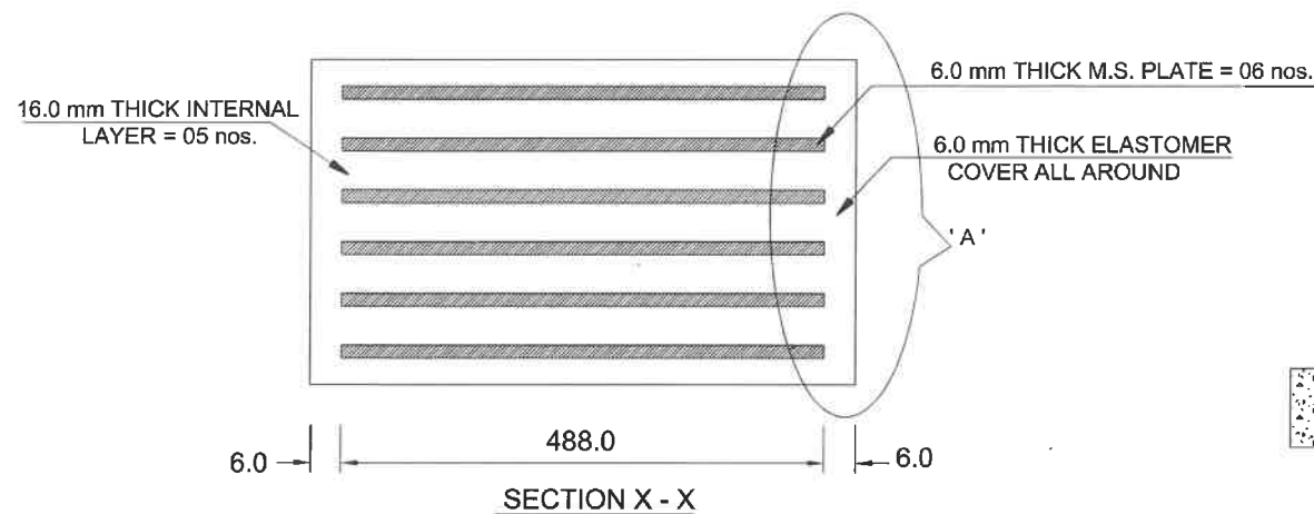
ARRANGEMENT OF BEARING AND PEDESTAL
