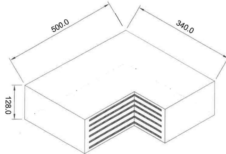
ISOMETRIC VIEW OF ELASTOMERIC BEARING ( TYP )
